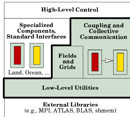
Figure 2: ESMF Application Architecture
